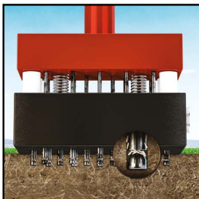
Seed filled spikes extended.
